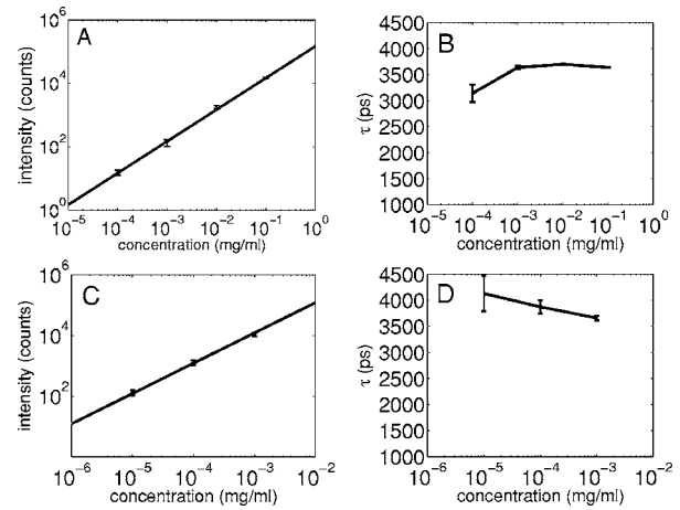
Fig. 2 Measured fluorescence signal rises monotonically with an increased fluorophore concentration. At higher laser attenuation (Panel A), the background autofluorescence was not subtracted and intensity varied linearly over 4 orders of magnitude. The lifetime (Panel B) was found to be very stable although it was found to be slightly lower with greater error at the lowest concentration. At a lower attenuation, the background autofluorescence was subtracted. The intensity was found to be linearly dependent on concentration (Panel C). The fitted lifetime did not vary significantly; the standard deviation increased at low concentrations but was small (Panel D). The amplitude of the fitted curve is shown to vary monotonically with respect to molarity. The background subtraction was performed on the data in Panels C and D. Lifetimes were found to be concentration-independent at 3747 \pm 3.3\% standard deviation, \chi^2 < 1.2 for all fits.
