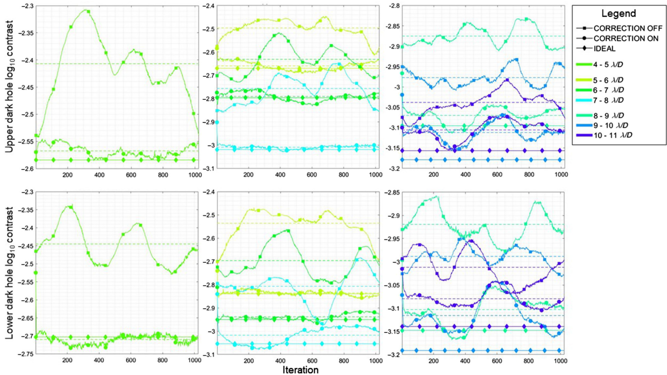
Fig. 20 Lab results showing the temporal evolution of contrast across 4 to 11 \lambda/D in 1 \lambda/D bins for both the upper and lower dark holes in the presence of an evolving phase aberration. The plots show the change in contrast in open-loop with no correction and in closed-loop with the LDFC-derived correction applied. The expected contrast under ideal conditions is also plotted for reference.
