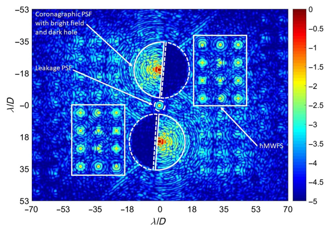
Fig. 1 Simulation example of the science image delivered by a vAPP coronagraph. Shown here are the two circularly polarized coronagraphic science PSFs each with a 2 to 15\lambda/D dark hole with an average contrast of \sim 10^{-5} and a bright field opposite the dark hole. Between the two coronagraphic PSFs is a leakage PSF that is generated by unpolarized light leakage in the vAPP. Located farther out in the image are 12 hMWFS PSFs each encoded with a single low-order Zernike mode.
