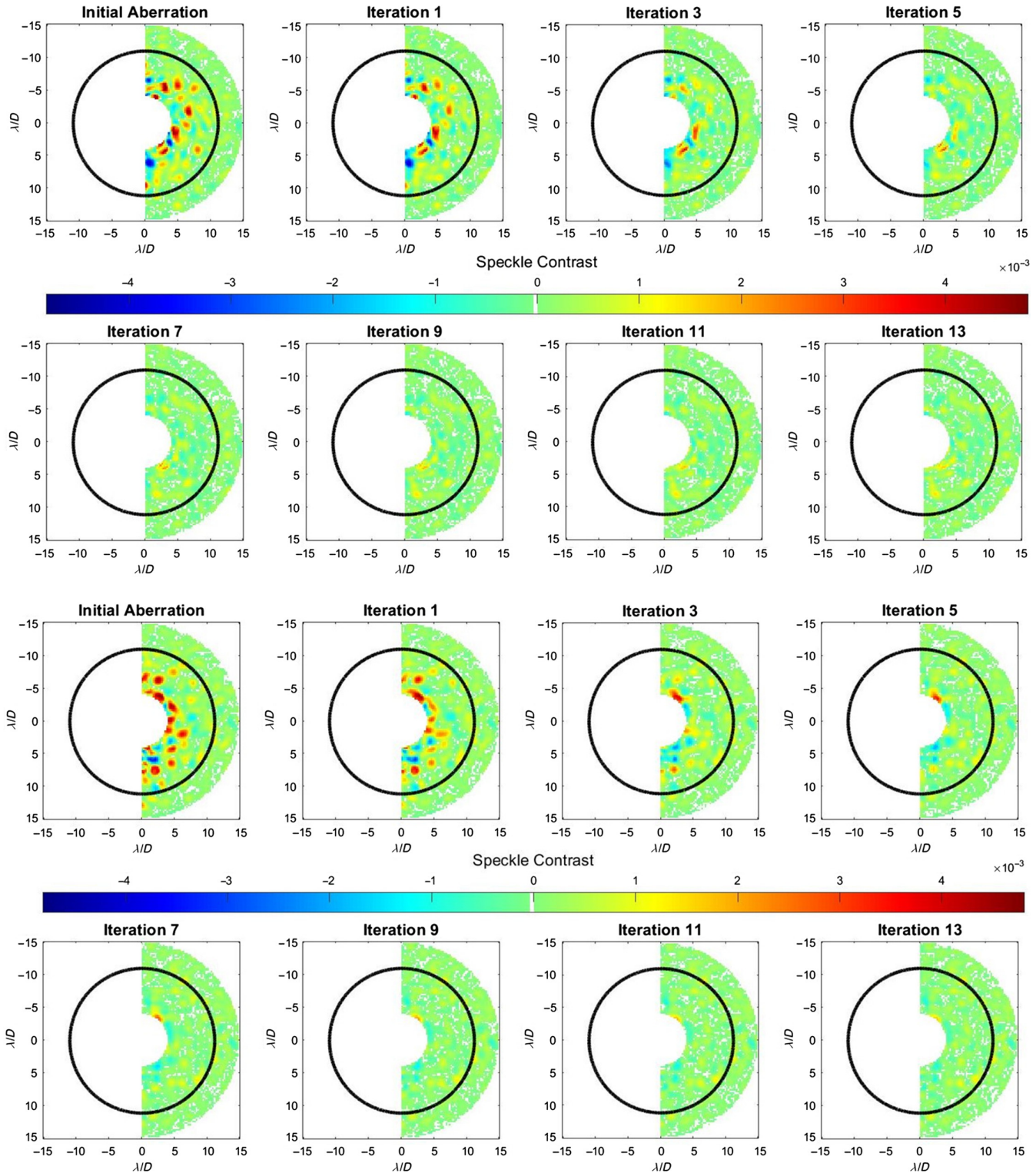
Fig. 21 Speckle suppression in the lab across the 4 to 15 \lambda/D dark hole returning the average contrast to the best achievable contrast level expected in the lab under ideal conditions. The black line denotes the control radius of the DM.
