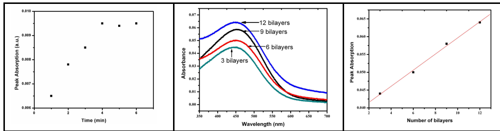
Fig. 2. (Left) Peak absorption of one bi-layer plotted against adsorption time, (middle) absorbance spectra of PDAC/H-PURET multilayers, and (right) peak absorption of PDAC/H-PURET with number of multilayers.
