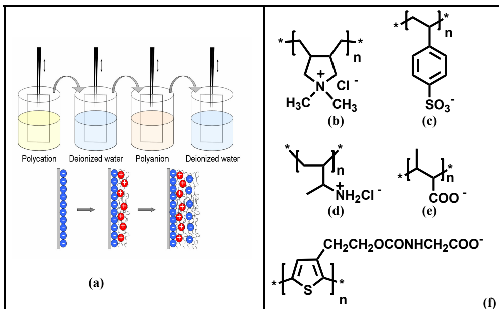
Fig. 1. (a) Schematic of LbL assembly process, and chemical formulas of (b) PDAC, (c) PSS, (d) PAH, (e) PAA and (f) H-PURET.
