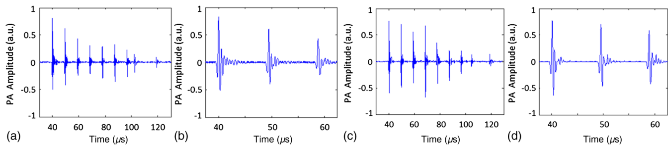
Fig. 6 Plots of acoustic waveforms propagating through the optical-fiber PADLs with various lengths ranging from 21 to 56 cm: (a) Raw A-line signals obtained by ultrasonic transducer UT1; (b) zoom-in view of the first three signals in (a); (c) raw A-line image obtained by ultrasonic transducer UT2; and (d) zoom-in view of the first three signals in (c).
