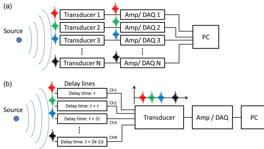
Fig. 1 (a) Photoacoustic (PA) signal reception using multiple transducers and multichannel data acquisition (DAQ) electronics; and (b) PA signal reception using a single-element transducer and single-channel DAQ electronics through parallel acoustic delay lines.
