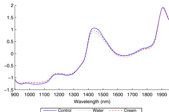
Fig. 2 Mean of the mean absorption graph of all volunteers before, and after application of a wet patch followed by a moisturizer.
