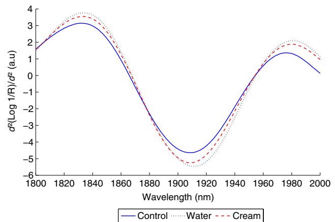
Fig. 9 Second derivative spectra of Group 1 for the three measurements recorded.
