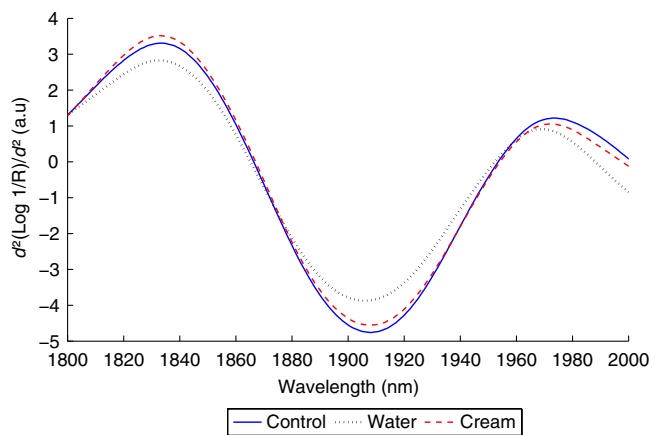
Fig. 11 Second derivative spectra of Group 3 for the three measurements recorded.
