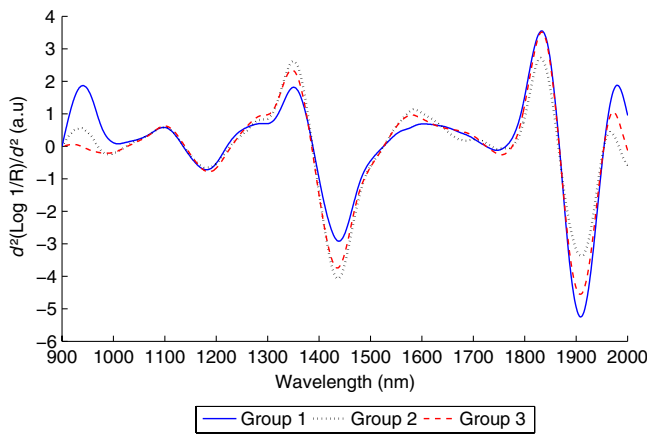
Fig. 8 Second derivative spectra after treatment with a cream. Response for Groups 1–3.
