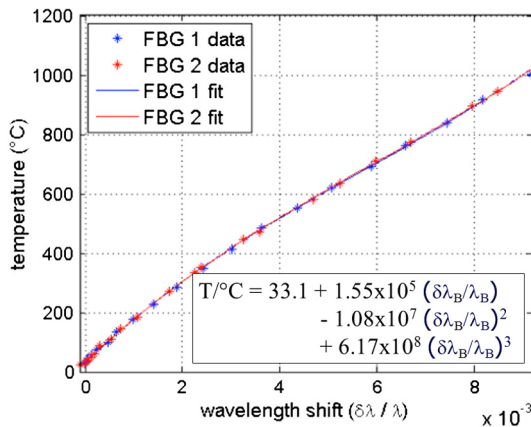
Fig. 6 Calibration curve for high-temperature FBGs deduced from the results in Fig. 5.
