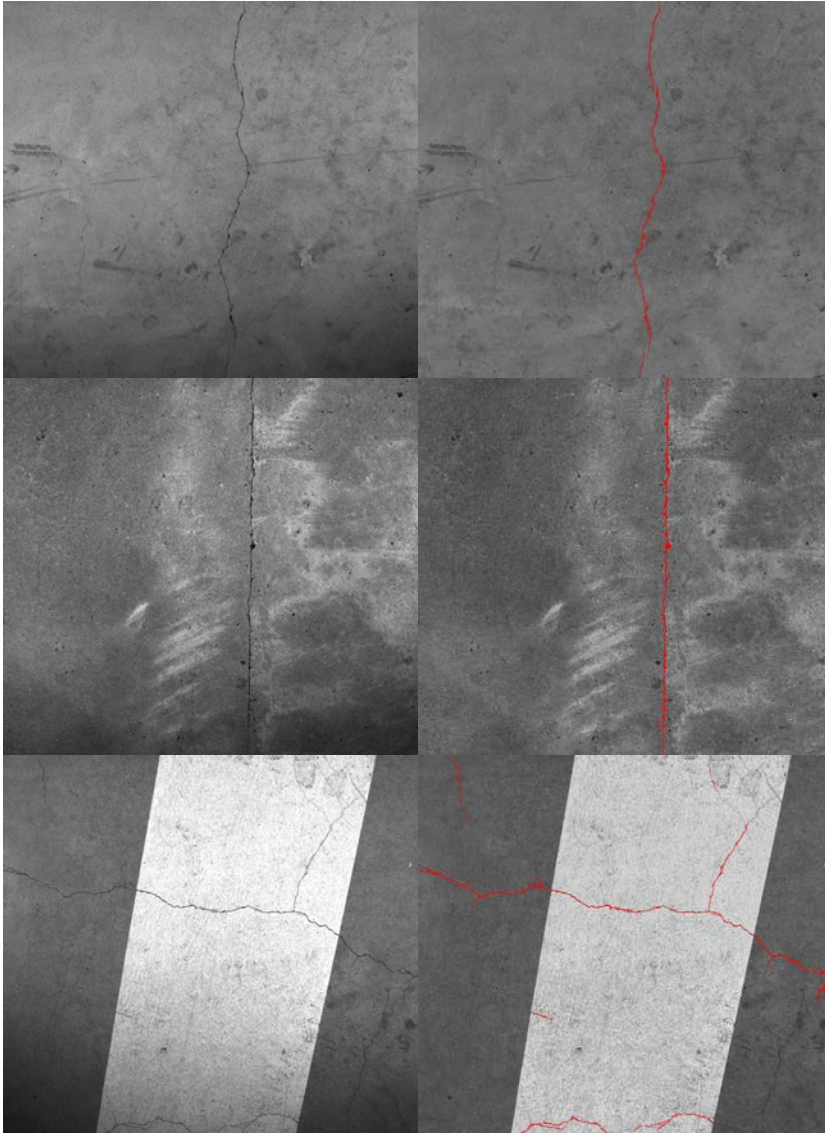
Figure 5: Left: input images containing various kinds of cracks with different widths, on different concrete floors. Right: crack map in red.
