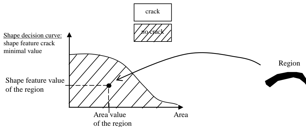
Figure 3: The size-dependent shape filter. In this example, the region is discarded. According to the classifier, its shape feature value is not high enough to be a crack.
