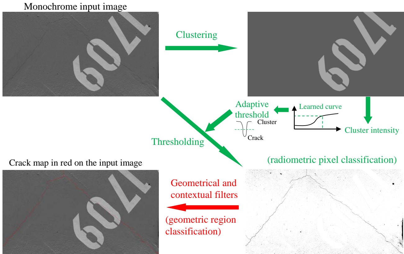
Figure 2: Flow chart of the crack detection algorithm. Comment of the result for this image: the crack is almost entirely detected in both clusters, and there is no false positive.
