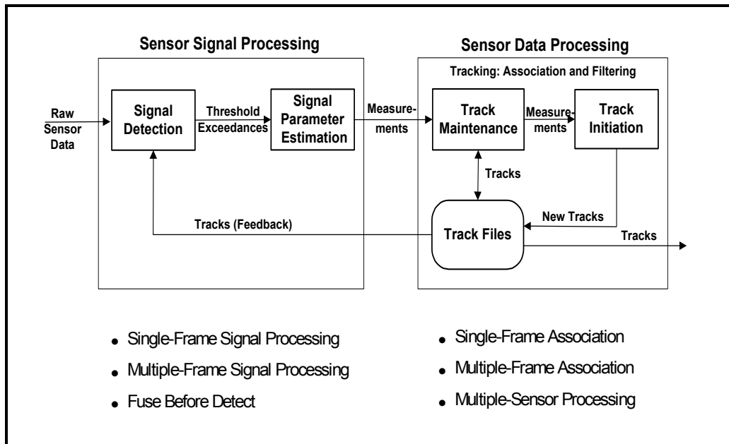
Figure 1. Sensor Signal and Data Processing
