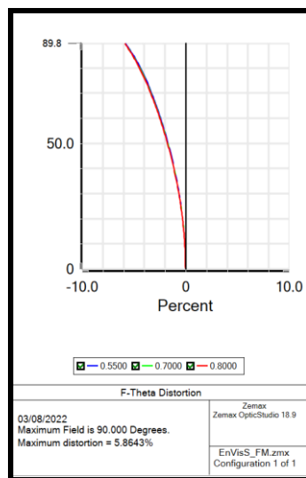
Figure 2-3: EnVisS nominal F \theta distortion.
