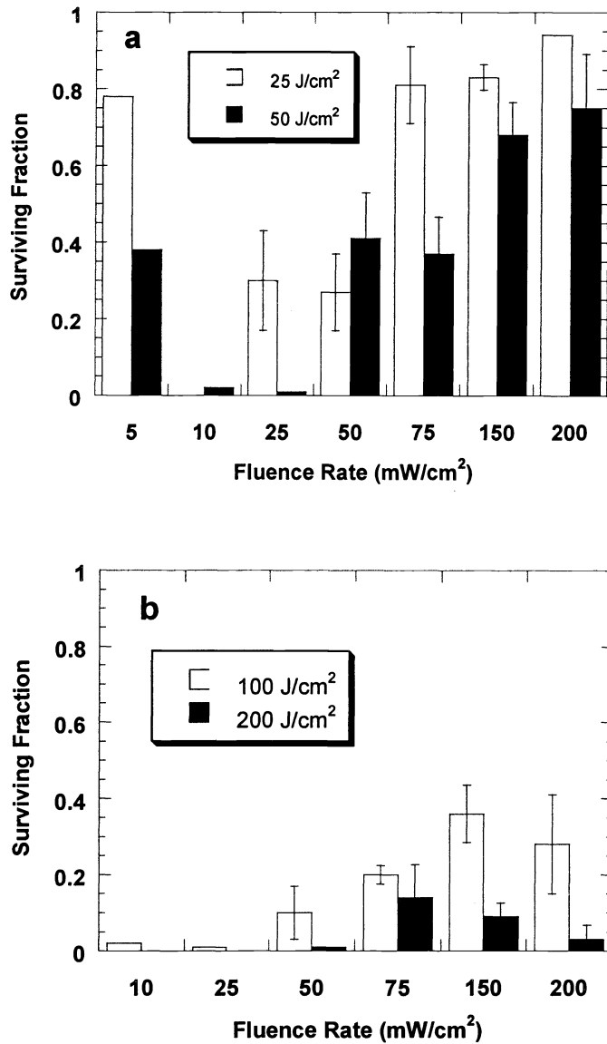
Figure 1. Spheroid survival as a function of fluence rate at representative fluences: (a) 25 and 50 J cm -2 ; and (b) 100 and 200 J cm -2 . Each data point represents the mean of approximately 40 spheroids. Standard errors are denoted by error bars.
