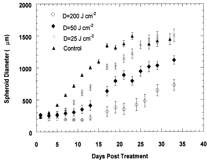
Figure 3. Growth kinetics of spheroids exposed to fluences of: 200, 50 and 25 \text{ J cm}^{-2} . A fluence rate of 75 \text{ mW cm}^{-2} was used in all cases. Each data point represents the mean of approximately 40 spheroids. Standard errors are denoted by error bars.
