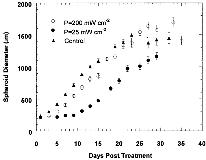
Figure 2. Growth kinetics of spheroids exposed to 25 \text{ J cm}^{-2} delivered at fluence rates of 25 and 200 \text{ mW cm}^{-2} . Each data point represents the mean of approximately 40 spheroids. Standard errors are denoted by error bars.
