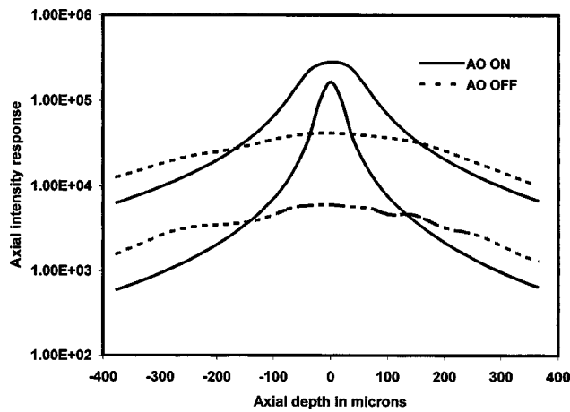
Fig. 2 Axial intensity responses with (solid lines) and without (dashed lines) AO. The bottom pair of lines is for a confocal pinhole diameter equal to the Airy disk radius of the light collection optics in the AOSLO (23 \mu\text{m} ), and the top pair of lines is for an 80- \mu\text{m} confocal pinhole. The subject had an initial r.m.s. wave aberration of 0.60 \mu\text{m} ; after AO correction it was reduced to 0.11 \mu\text{m} .
