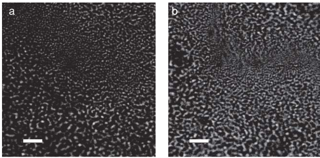
Fig. 2 White light transmission images of (a) S. mutans and (b) S. sanguinis show that the species cannot be distinguished based on appearance alone. (Bar length = 10 \mu\text{m} .)
