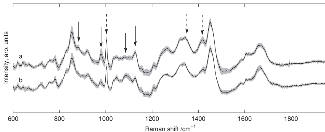
Fig. 3 Mean spectra from (a) S. sanguinis and (b) S. mutans used in the training set. Shaded regions show the standard deviation for each species. Arrows highlight regions useful in species classification as flagged by LR; solid arrows indicate features used for peak-based discrimination.
