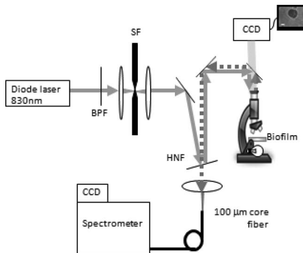
Fig. 1 Schematic overview of confocal Raman microscope; see text for details. Abbreviations: BPF, bandpass filter; SF, spatial filter; HNF, holographic notch filter.
