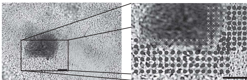
Fig. 4 White light transmission image of pseudo-mixed biofilm (left) with a close-up of the scanned region (right). Darker regions are S. sanguinis stained with CV, while lighter regions are unstained S. mutans . Assignments in the scan: dark circles, S. mutans ; light circles, S. sanguinis ; x, spectral outlier (for example, due to the stain). Circle sizes represent laser focus. (Bar length = 10 \mu\text{m} .)
