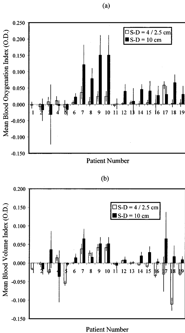
Fig. 4 Mean and standard deviation of (a) the blood oxygenation index and (b) the blood volume index, quantified from NIR measurements made at both the 10 and 4/2.5 cm source-detector separations on the mid line of the maternal abdomen, during the NST period.
