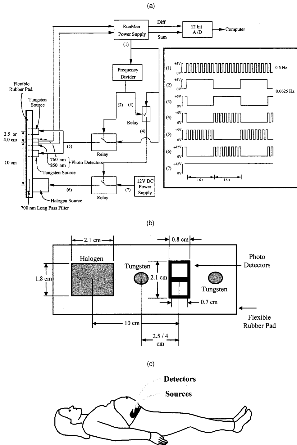
Fig. 1 A schematic of (a) the cw, NIR spectrometer, (b) the corresponding optical probe, which contains two source-detector pairs, and (c) its placement on the maternal abdomen.
