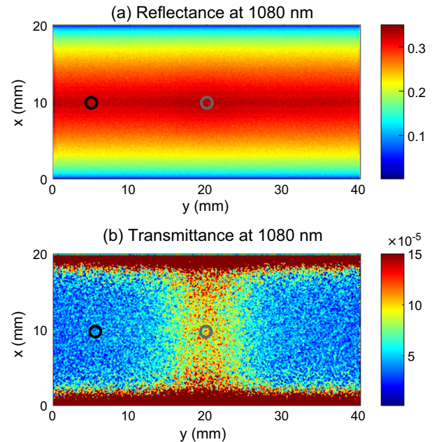
Fig. 4 (a) Reflectance and (b) transmittance image of the normal finger model at 1080 nm. Circles mark the areas from which the spectra presented in Fig. 4 were obtained (black–bone area, gray–cavity area).
