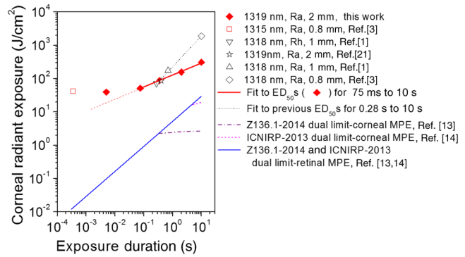
Fig. 3 Corneal damage thresholds determined in our experiment and reported by previous investigations, and MPEs from ANSI Z136.1-2014 and ICNIRP-2013 for 1319 nm. 1,3,13,14,21 The 5-ms point was transformed from that at 1338 nm. The solid line was a least square fit to a power law, ED_{50} = 128.9t^{0.36} ( R = 0.997 ).
