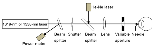
Fig. 2 Experimental setup.
