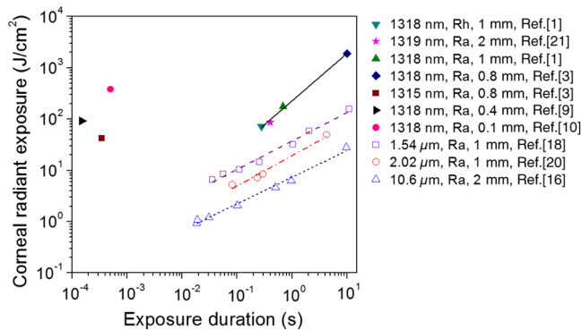
Fig. 1 Previous corneal damage thresholds ( ED_{50} or H_{th} ) in terms of J/cm^2 . 1,3,9,10,16,18,20,21 The parameters behind the symbols denote the laser wavelength, the animal species (Rh: Rhesus; Ra: Rabbit), and the corneal spot diameter. The four lines are the least square fits to damage thresholds: solid line: ED_{50} = 225.9t^{0.92} ( R = 0.997 ); dashed line: H_{th} = 37.3t^{0.55} ( R = 0.998 ); dashed-dotted line: H_{th} = 19.4t^{0.59} ( R = 0.983 ); and shot-dotted line: H_{th} = 7.36t^{0.52} ( R = 0.995 ).
