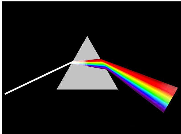
Figure 1.2 Newton's prism experiment.
